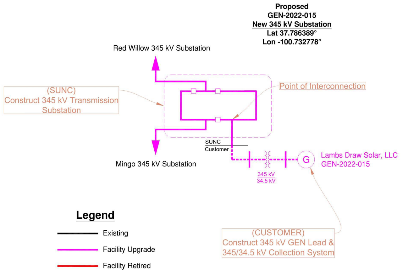
Figure 1: One-line Diagram Facilities for GEN-2022-015
